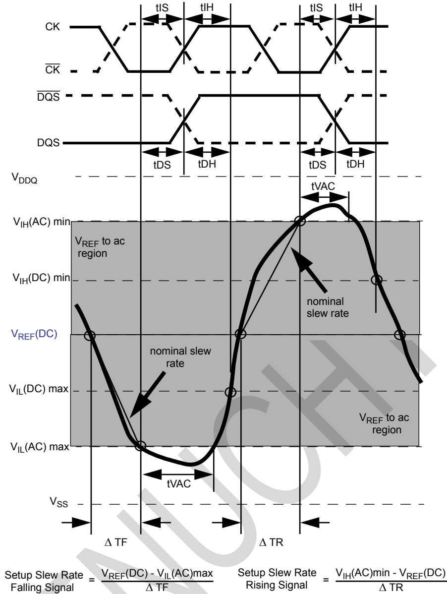
Figure 21. Illustration of nominal slew rate and t_{VAC} for setup time t_{DS} (for DQ with respect to strobe) and t_{1S} (for ADD/CMD with respect to clock).
