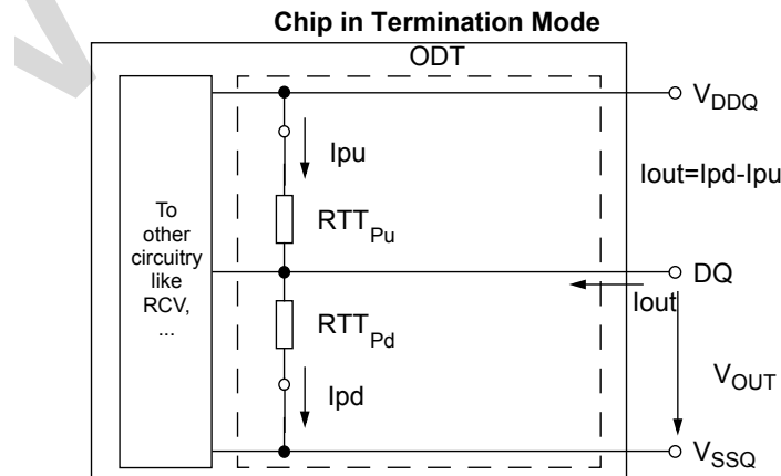
Figure 12. On-Die Termination : Definition of Voltages and Currents
