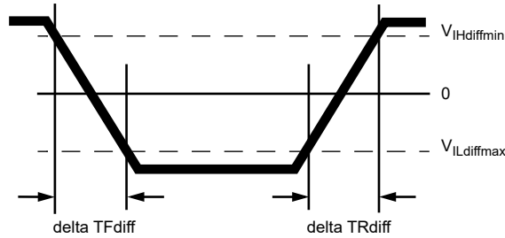
Figure 5. Differential Input Slew Rate definition for DQS, \overline{\text{DQS}} , and C, \overline{\text{C}}
