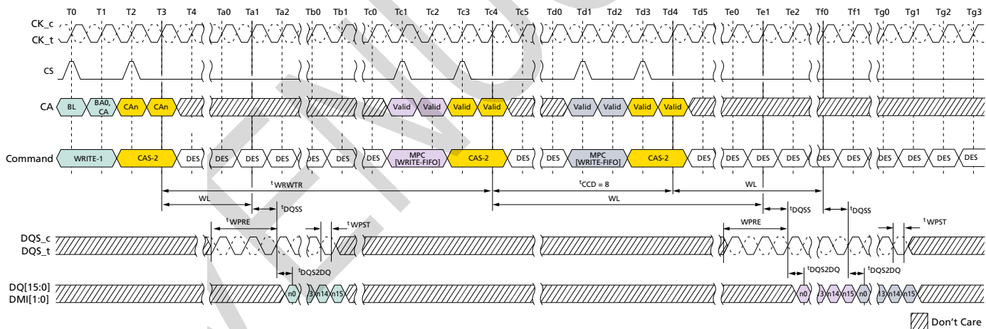
Figure 120: WRITE-FIFO – t_{WPST} = 2nCK , t_{WPST} = 0.5nCK
