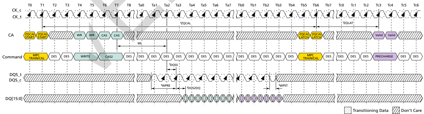
Figure 135: ZQCAL Timing
