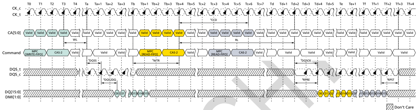
Figure 121: READ-FIFO – t_{WPRE} = 2nCK , t_{WPST} = 0.5nCK , t_{RPRE} = \text{Toggle} , t_{RPST} = 1.5nCK
