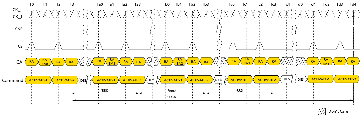
Figure 13: t_{FAW} Timing
