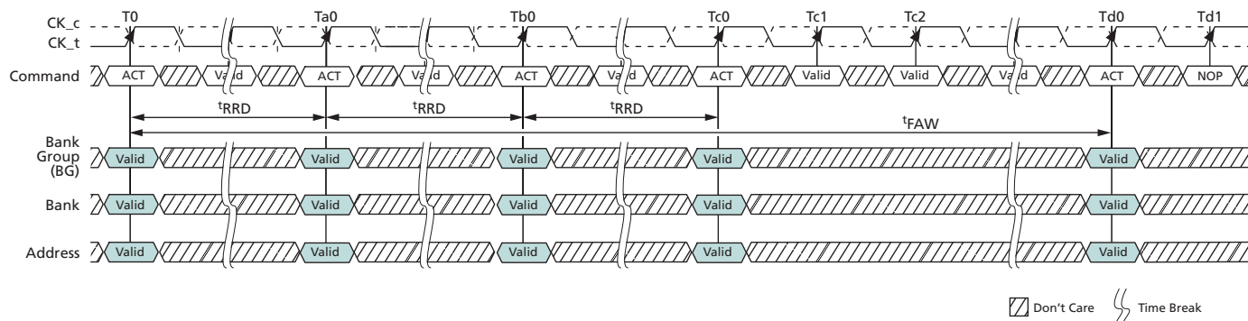
Figure 82: t^{\text{FAW}} Timing
