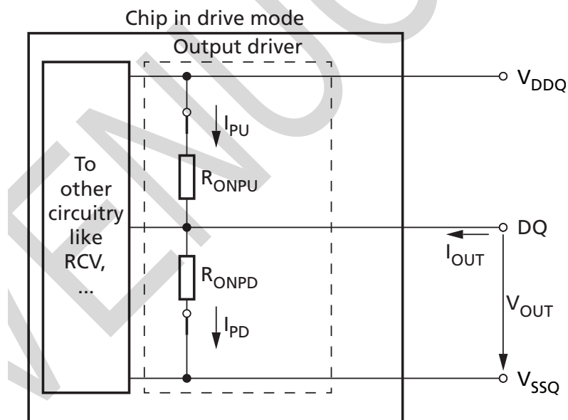
Figure 237: Output Driver: Definition of Voltages and Currents
