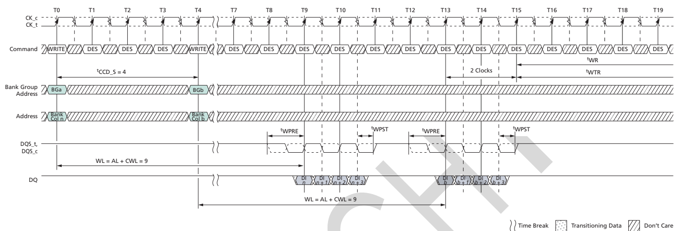
Figure 180: WRITE (BC4) Fixed to WRITE (BC4) Fixed with 1^{\text{tCK}} Preamble in Different Bank Group
