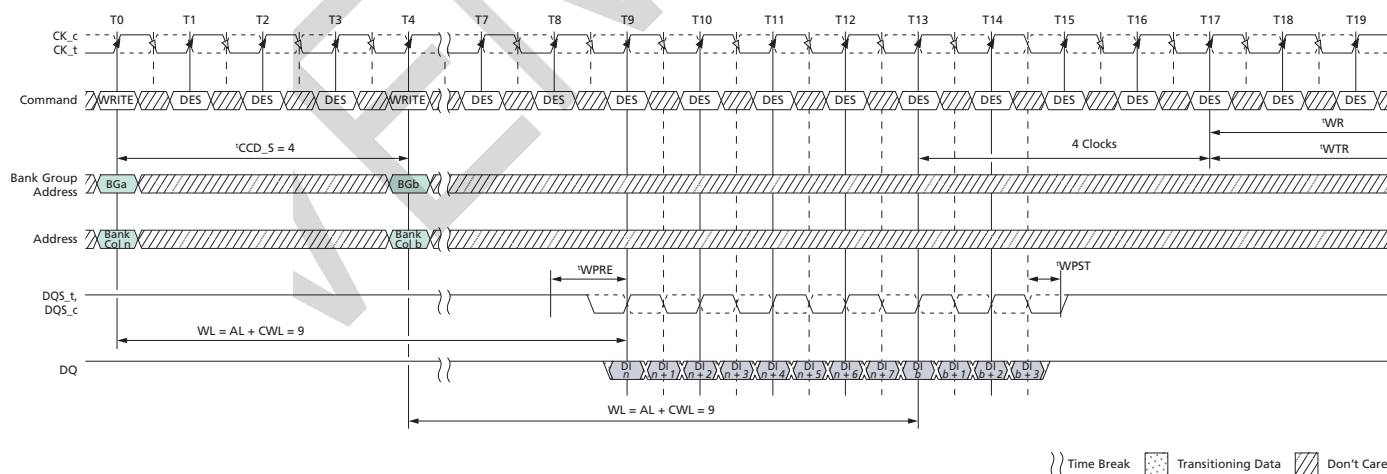
Figure 181: WRITE (BL8) to WRITE (BC4) OTF with 1^{\text{tCK}} Preamble in Different Bank Group
