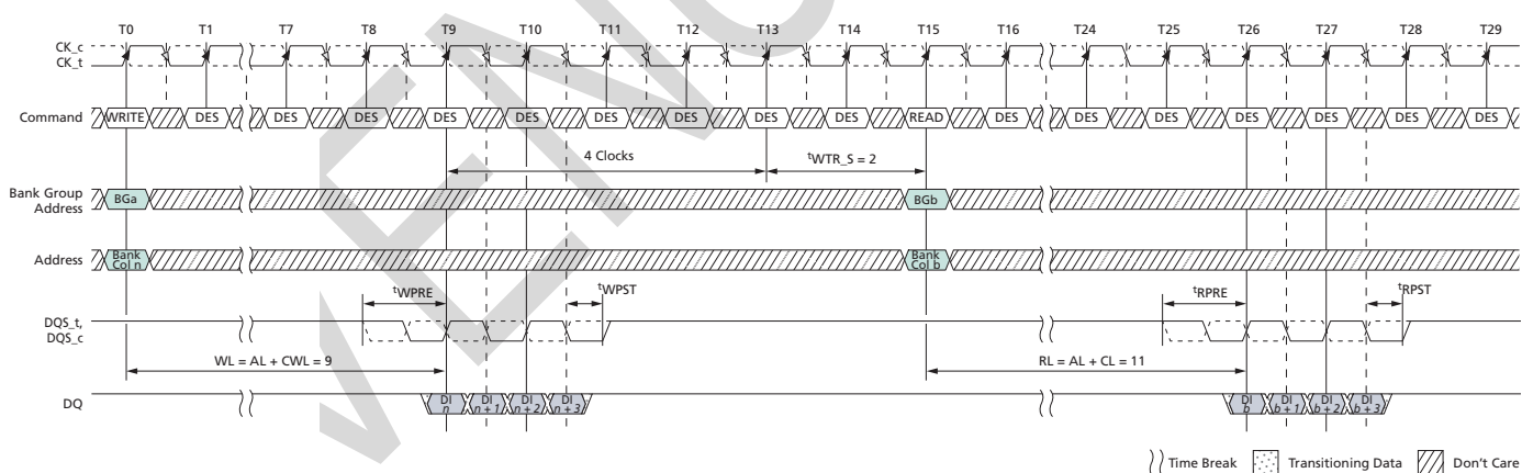
Figure 185: WRITE (BC4) OTF to READ (BC4) OTF with 1^{\text{t}}\text{CK} Preamble in Different Bank Group
