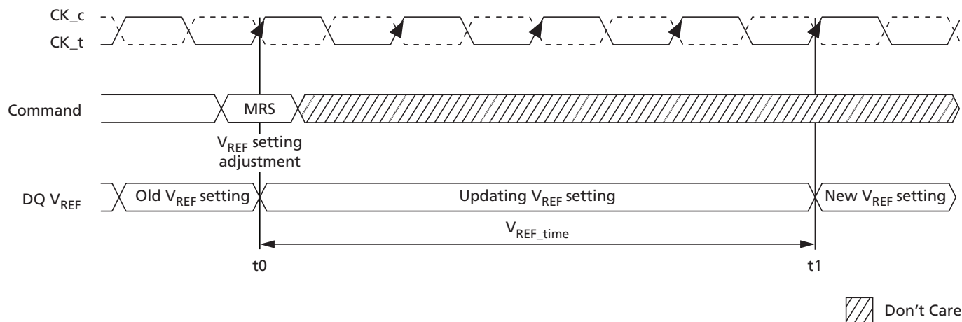
Figure 66: V_{REFDQ} Timing Diagram for V_{REF,time} Parameter
