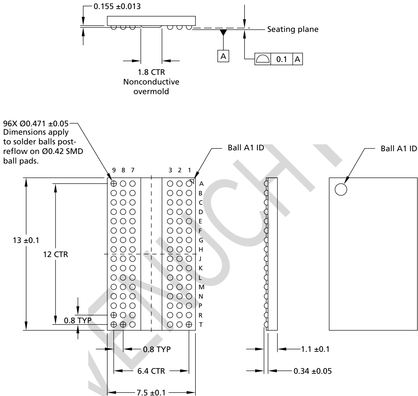
Figure 12: 96-Ball FBGA – x16 (TB)
