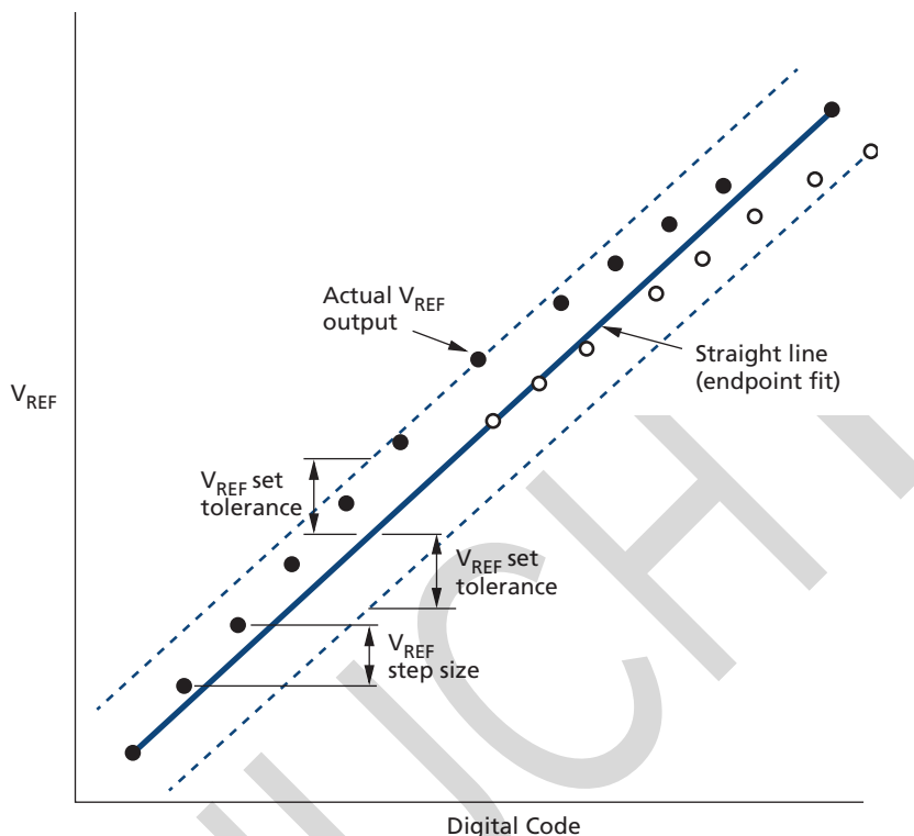
Figure 65: Example of V_{REF} Set Tolerance and Step Size
