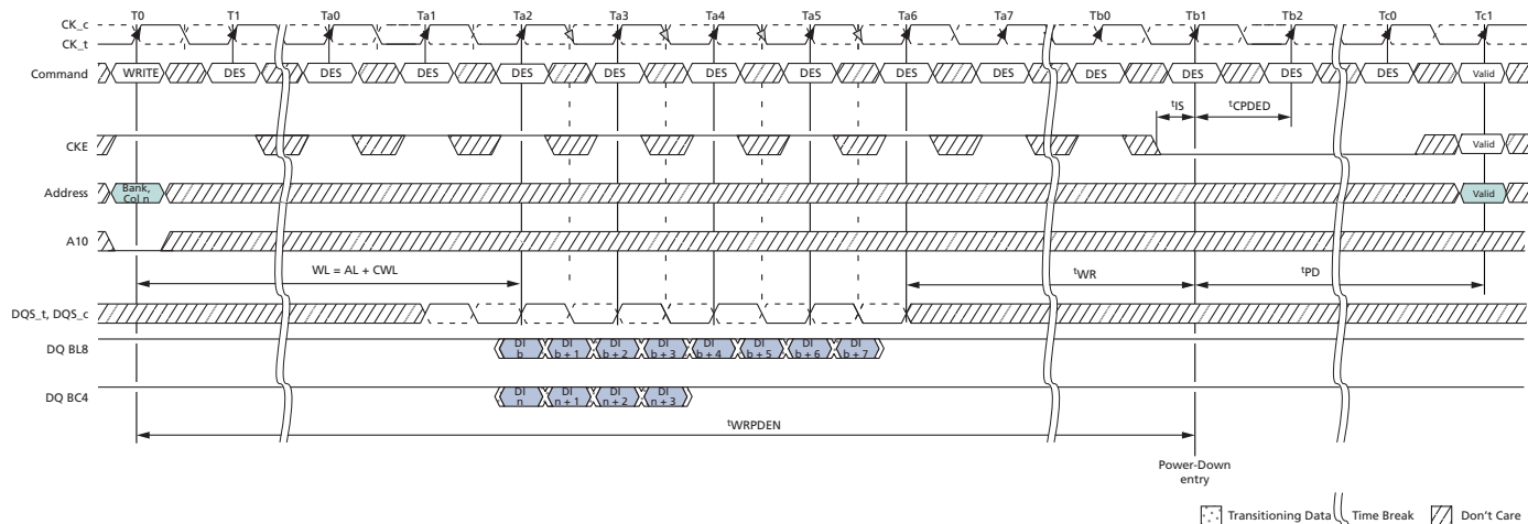
Figure 96: Power-Down Entry After Write
