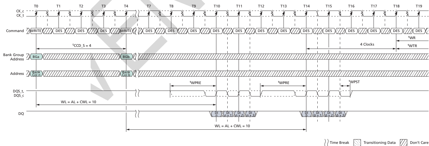
Figure 179: WRITE (BC4) OTF to WRITE (BC4) OTF with 2^tCK Preamble in Different Bank Group
