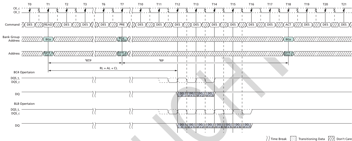
Figure 152: READ to PRECHARGE with 1^{th} CK Preamble
