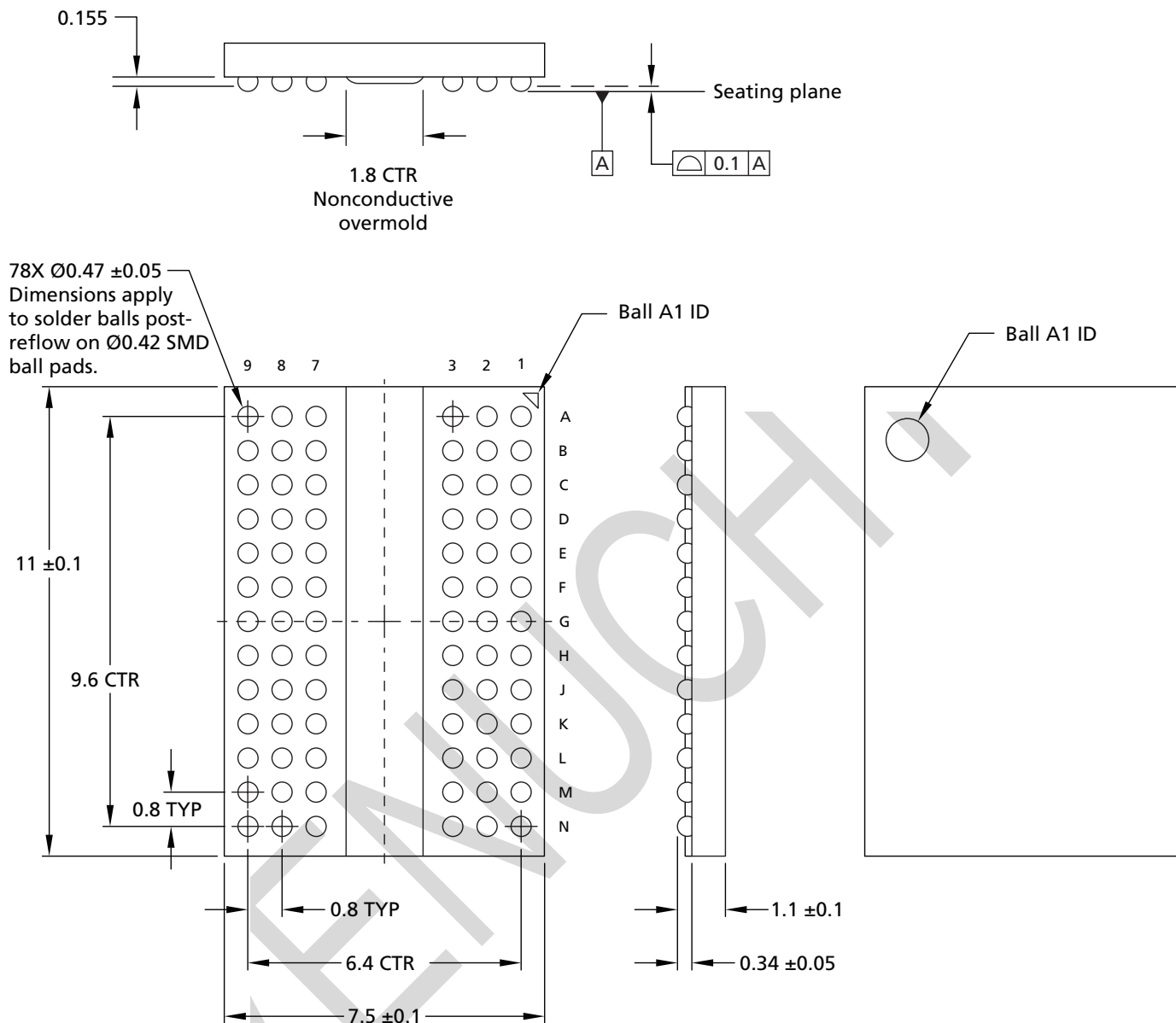
Figure 9: 78-Ball FBGA – x4, x8 (SA)
