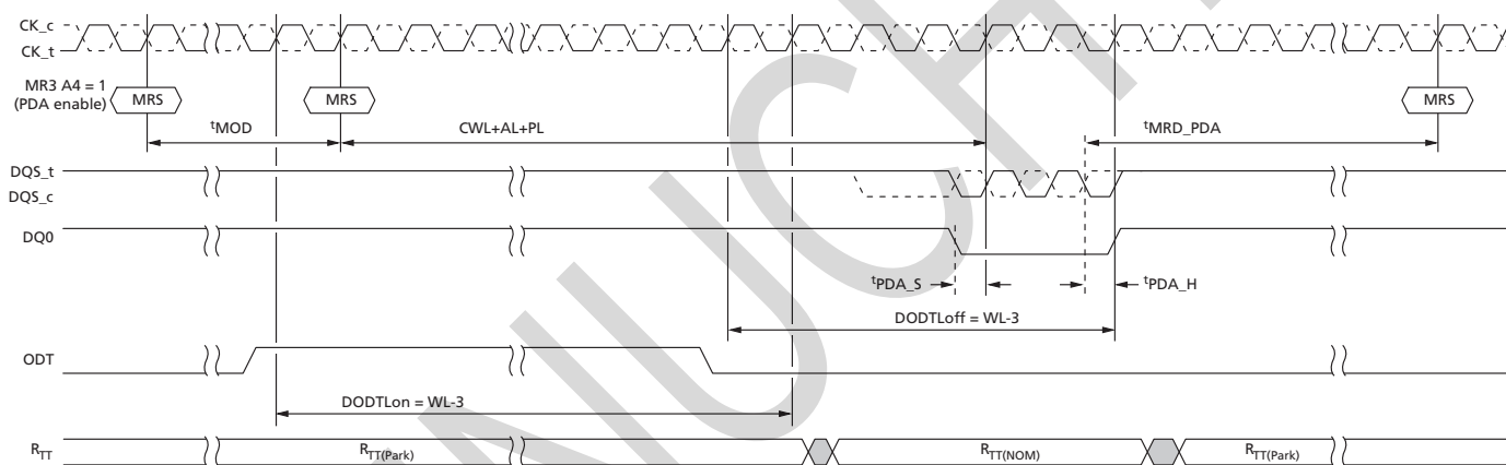
Figure 62: PDA Operation Enabled, BC4
