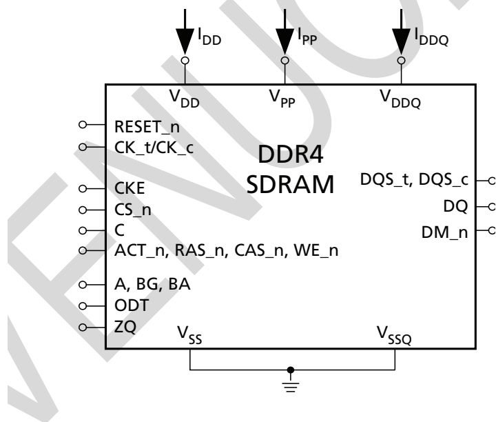
Figure 245: Measurement Setup and Test Load for I_{DDx} , I_{PPx} , and I_{DDQx}
