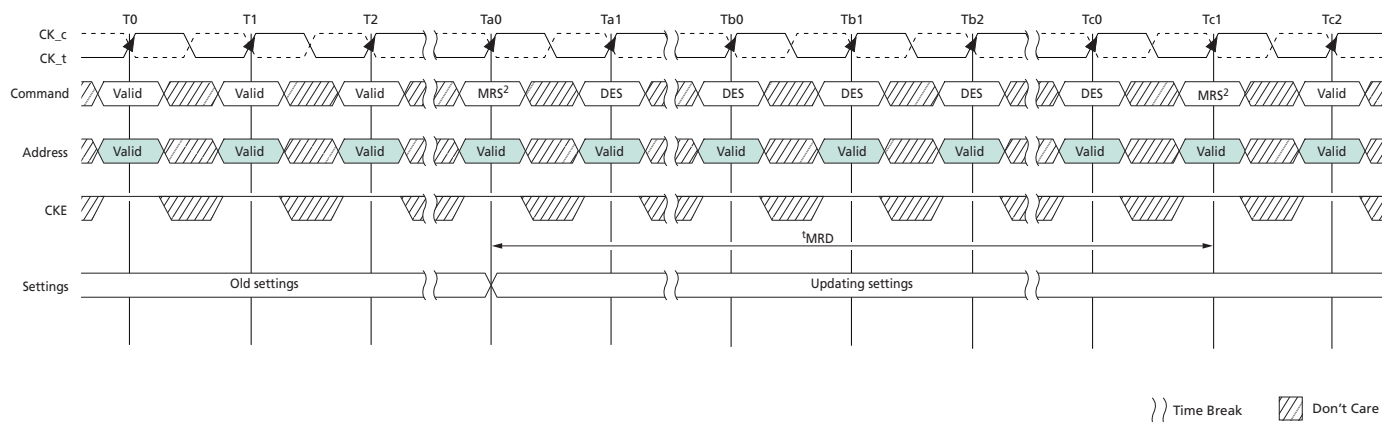
Figure 16: t^{\text{MRD}} Timing
