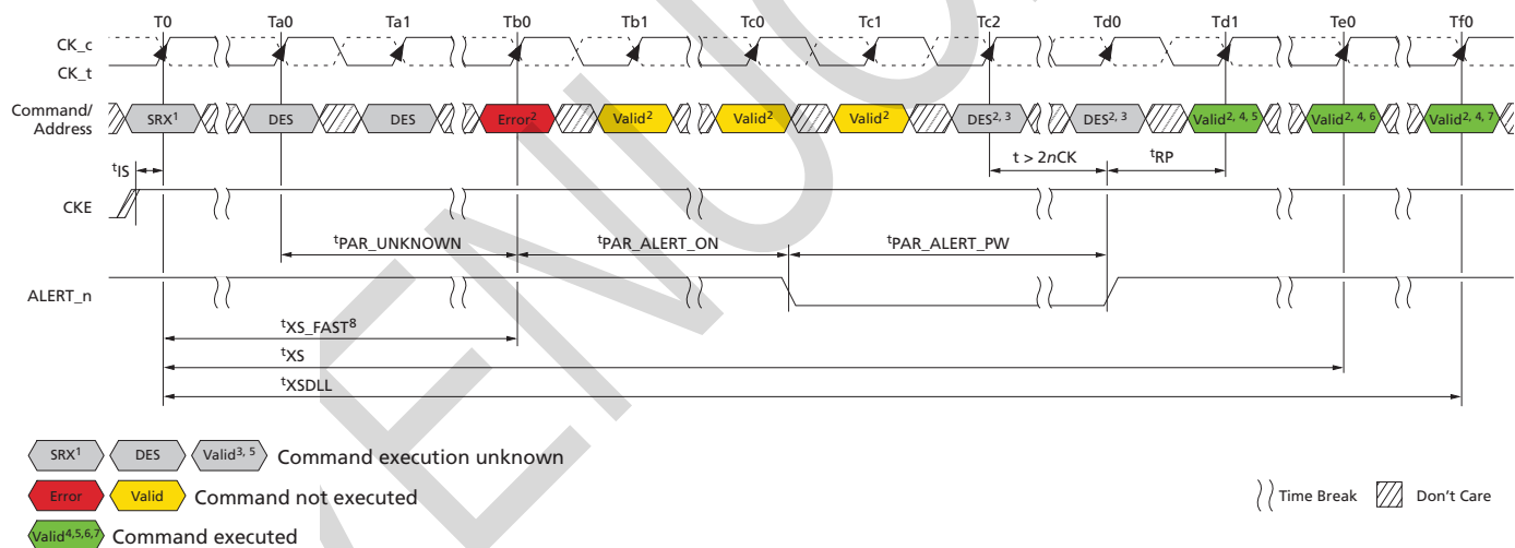
Figure 54: CA Parity Error Checking – SRX Attempt
