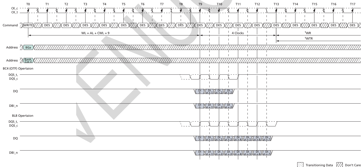
Figure 193: WRITE (BL8/BC4-OTF) with 1^t\text{CK} Preamble and DBI
