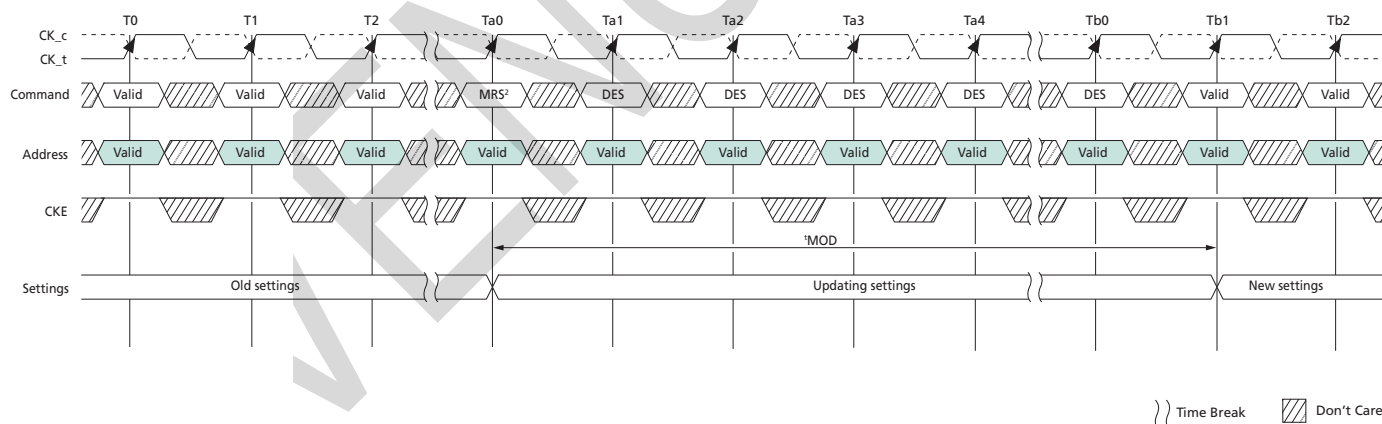
Figure 17: t^{\text{MOD}} Timing
