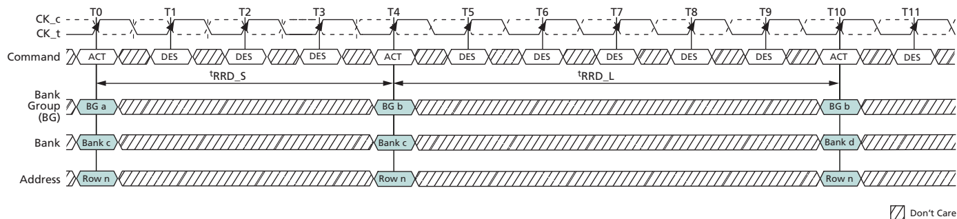
Figure 121: t_{RRD} Timing
