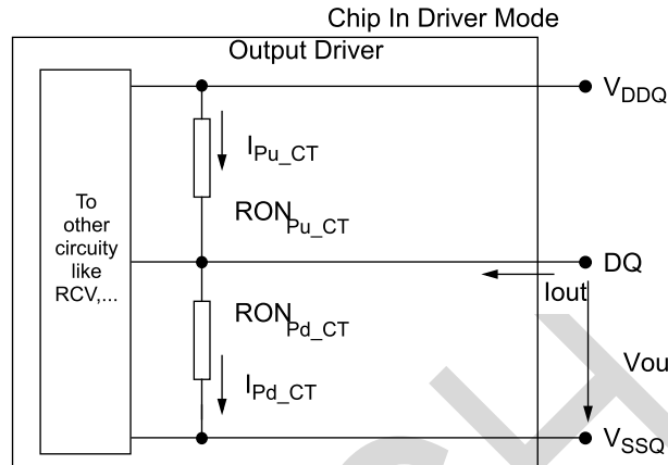
Figure 16. Output Driver
