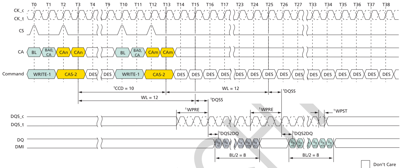
Figur 57: Consecutiv WRITE: t_{CCD} = \text{MIN} + 2, 0.5n\text{CK} Postamble
