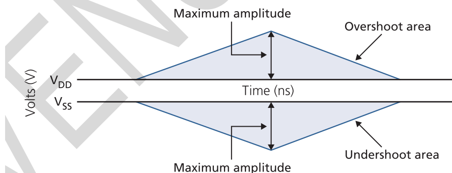
Figure 161: Overshoot and Undershoot Definition
