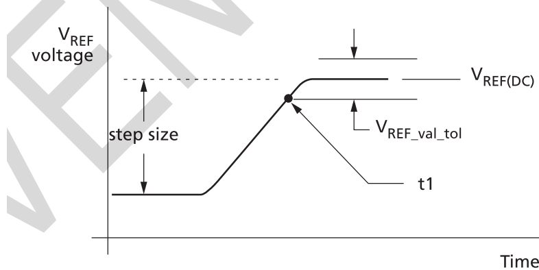
Figure 108: V_{REF(DQ)} Single-Step Size Increment
