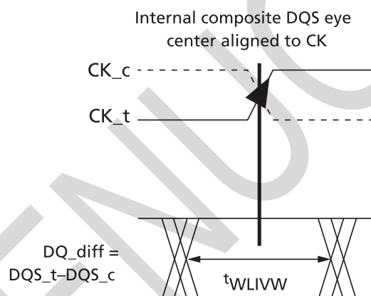
Figure 119: DQS_ t/DQS_ c to CK_ t/CK_ c Timings at the Pins Referenced from the Internal Latch
