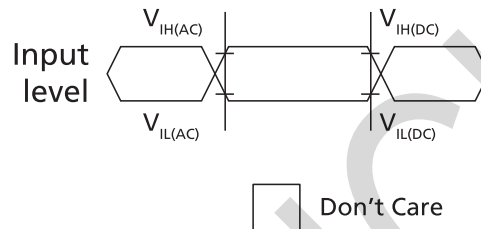
Figure 147: Input Timing Definition for CKE
