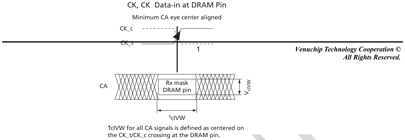
Figure 169: CA Timings at the DRAM Pins
