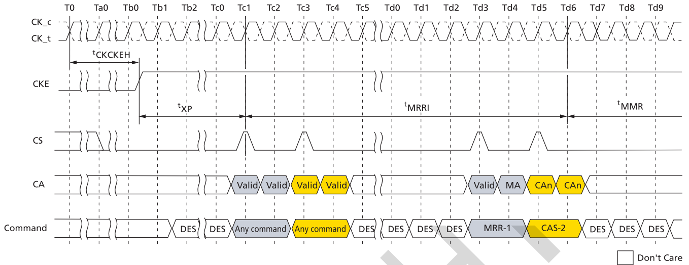
Figure 94: MRR Following Power-Down
