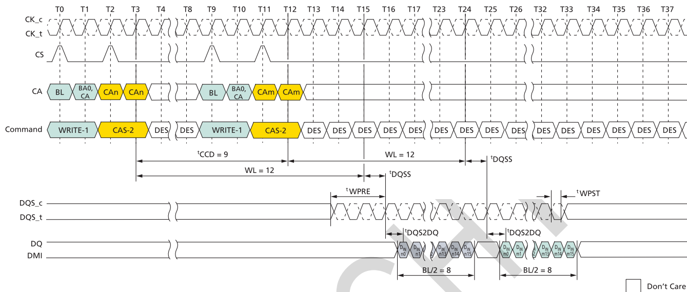
Figure 55: Consecutive WRITE: t_{CCD} = \text{MIN} + 1, 0.5nCK Postamble
