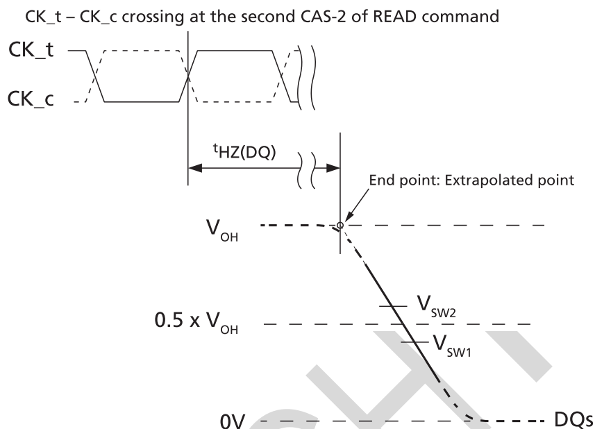
Figure 25: t_{HZ}(DQ) Method for Calculating Transitions and Endpoint
