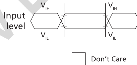
Figure 148: Input Timing Definition for RESET_n
