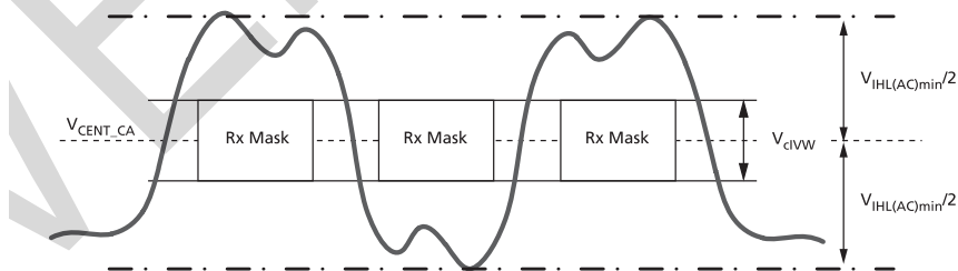
Figure 171: CA V_{IHL\_AC} Definition (for Each Input Pulse)
