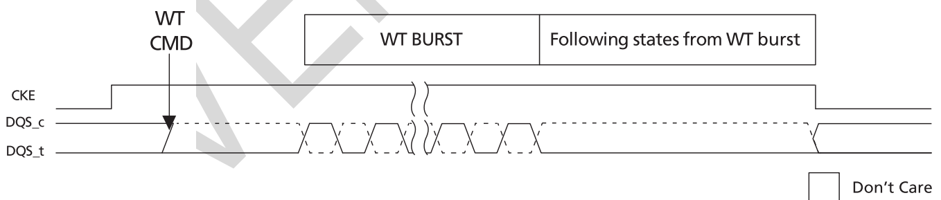
Figure 35: WDQS Control Mode 1
