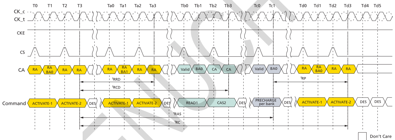
Figure 12: ACTIVATE Command
