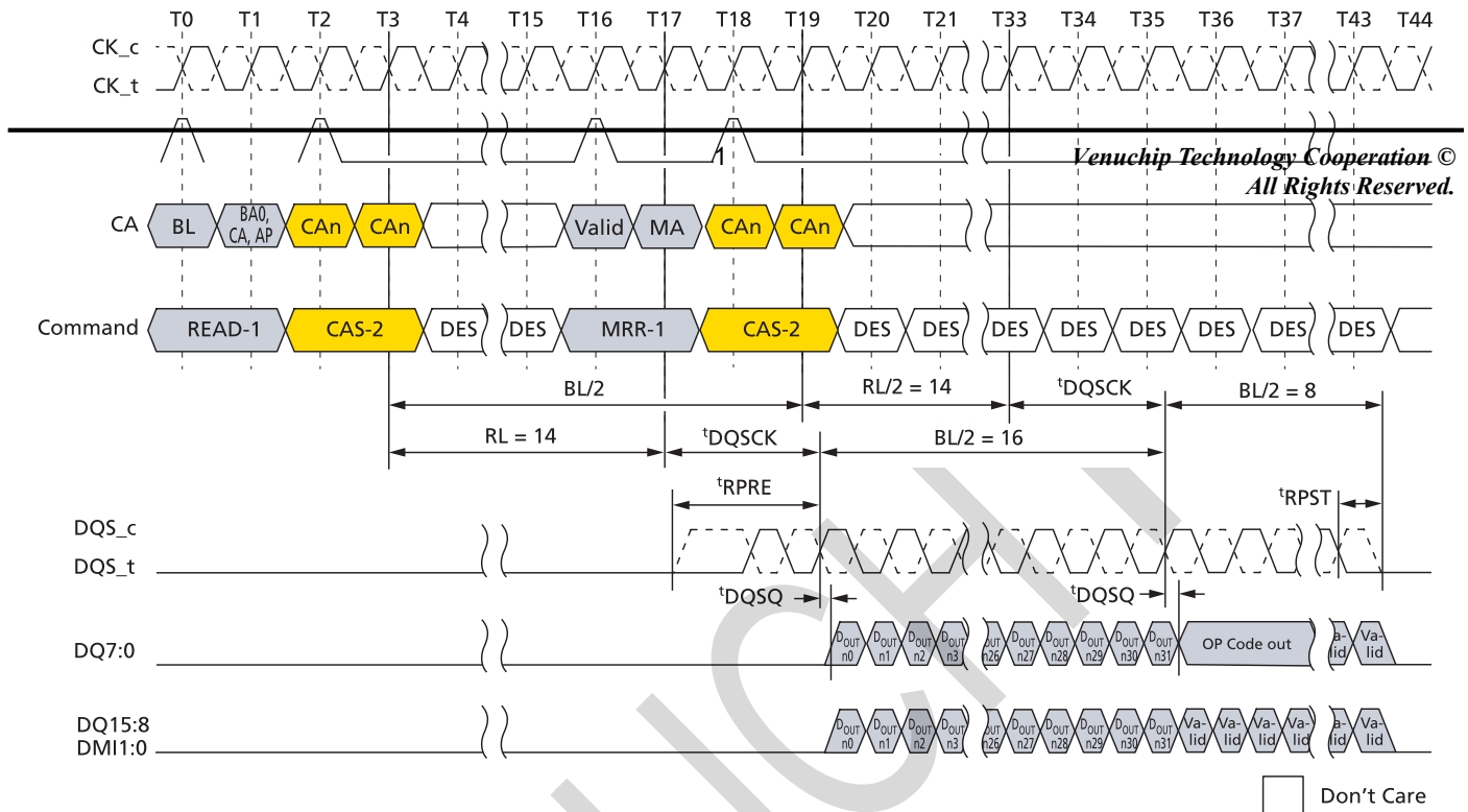
Figure 92: READ-to-MRR Timing
