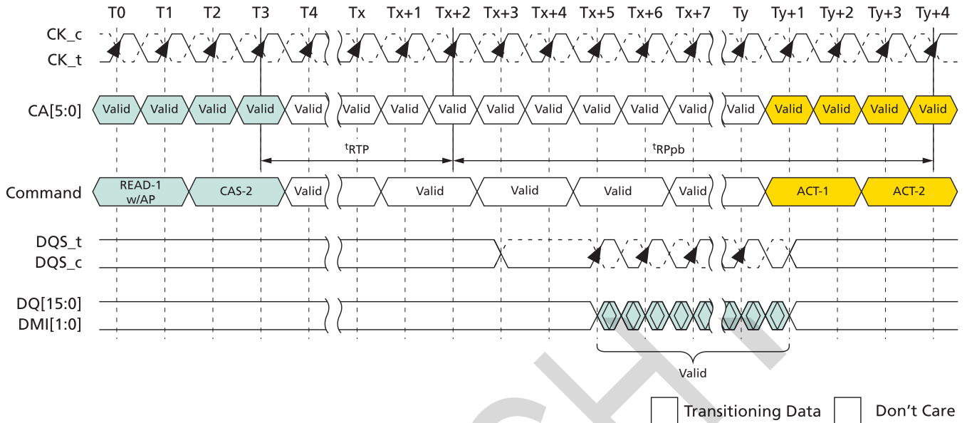
Figure 65: Burst READ With Auto Precharge – BL16, Non-Toggling Preamble, 0.5nCK Postamble
