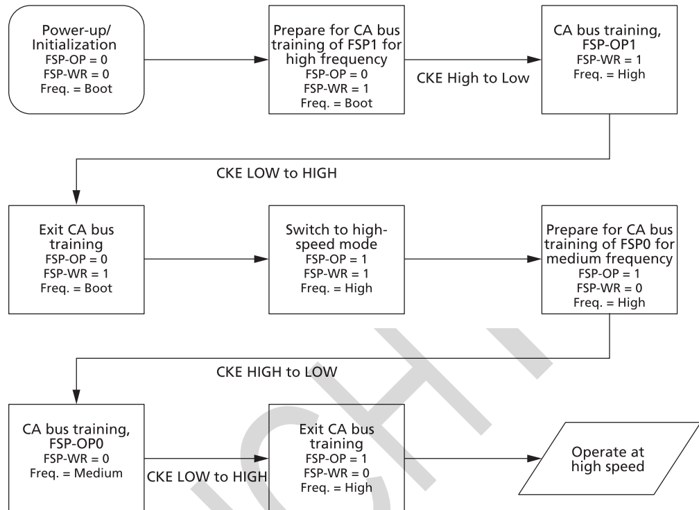
Figure 137: Training for Two Frequency Set Points
