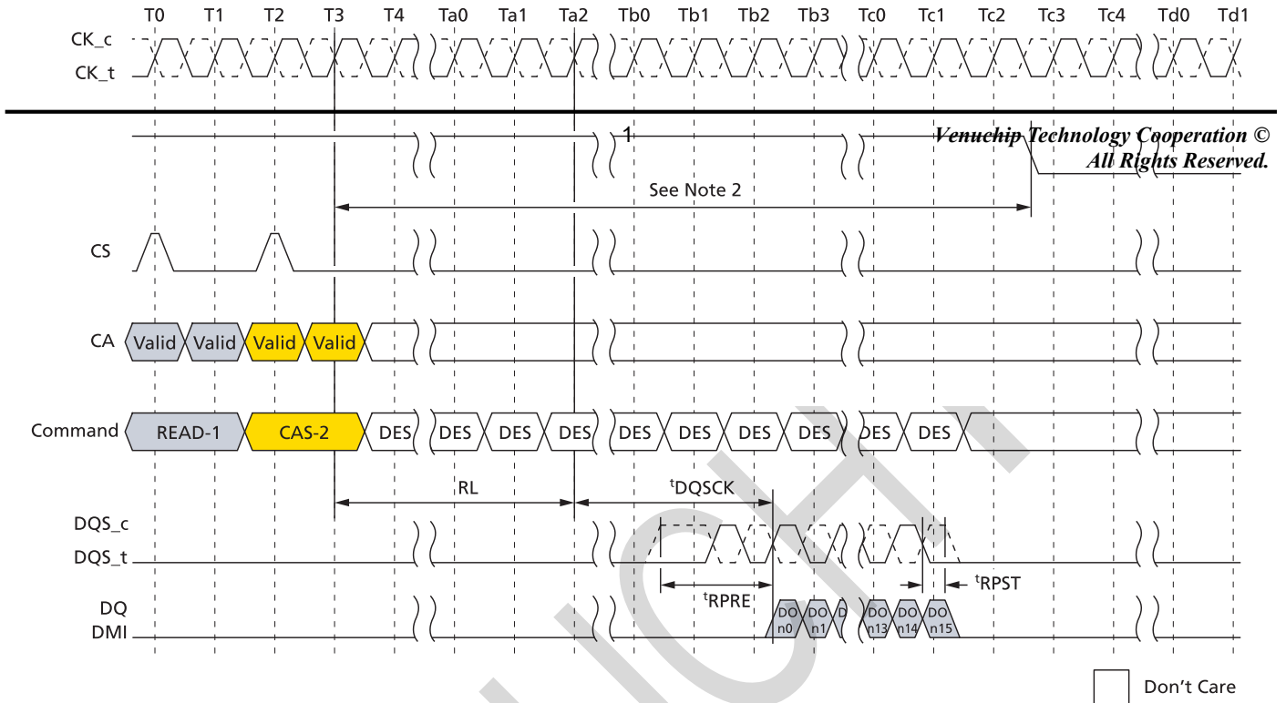
Figure 82: Read and Read with Auto Precharge to Power-Down Entry
