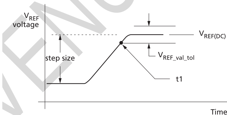
Figure 101: V_{REF(CA)} Single-Step Increment
