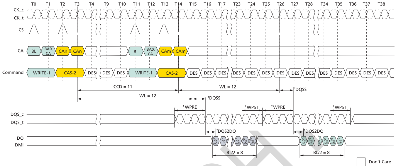
Figure 60: Consecutive WRITE: t_{CCD} = \text{MIN} + 3, 1.5nCK Postamble
