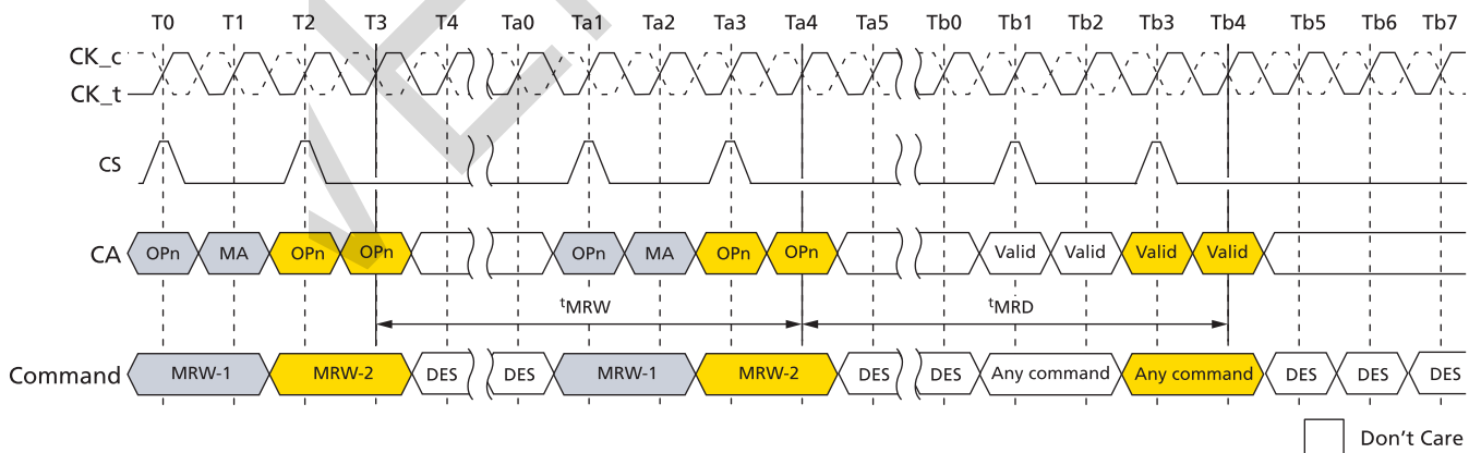
Figure 95: MODE REGISTER WRITE Timing
