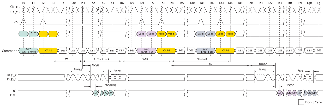
Figure 127: MPC[WRITE-FIFO]-to-MPC[READ-FIFO] Timing
