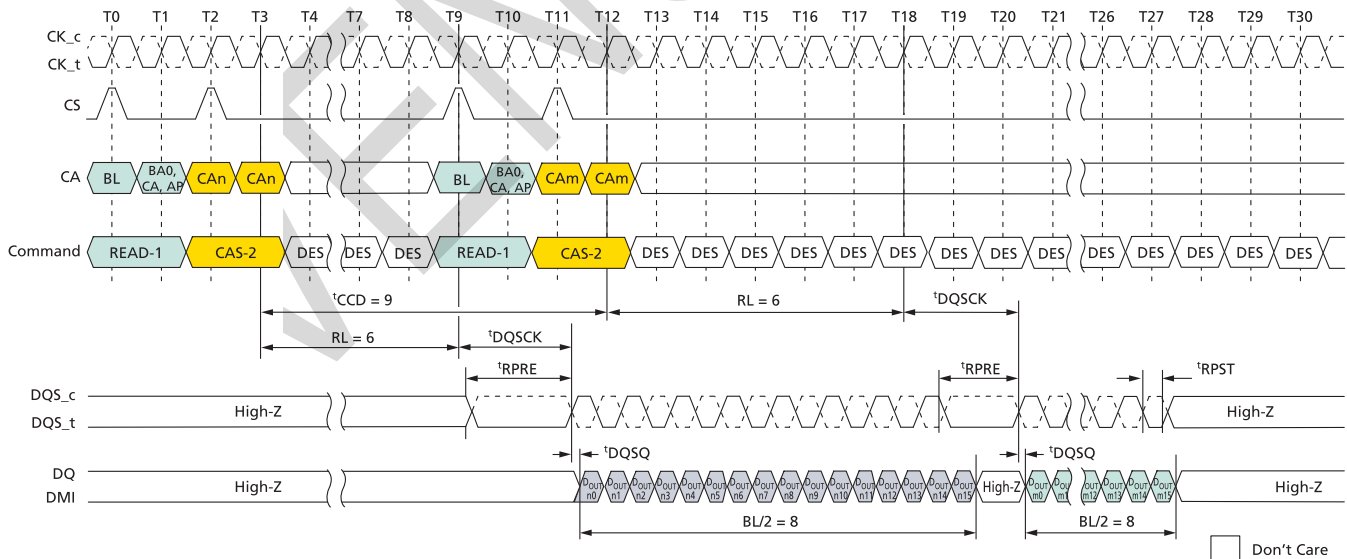
Figure 43: Consecutive READ: t_{\text{CCD}} = \text{MIN} + 1 , Preamble = Static, 0.5n\text{CK} Postamble
