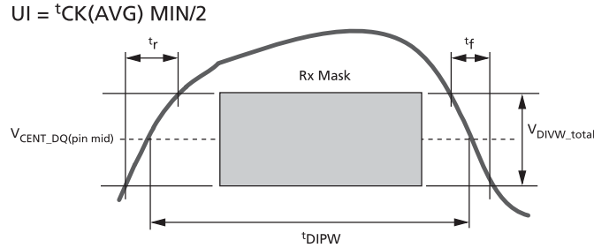
Figure 176: DQ DIPW and SRIN_divW Definition for Each Input Pulse
