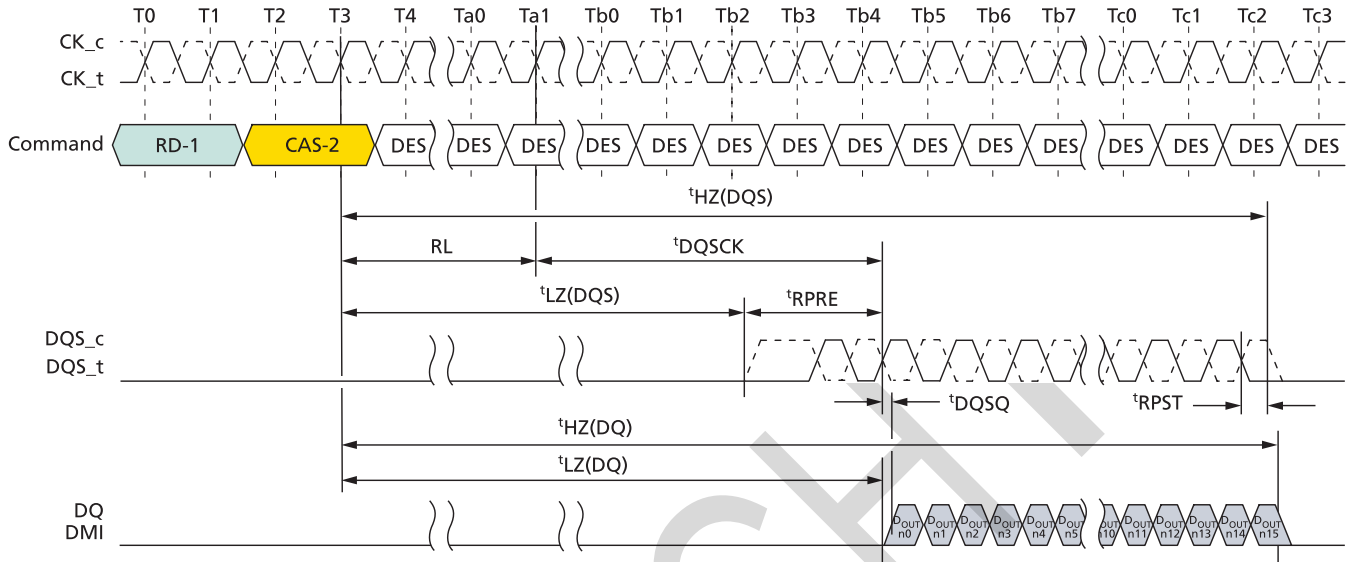
Figure 21: Read Timing
