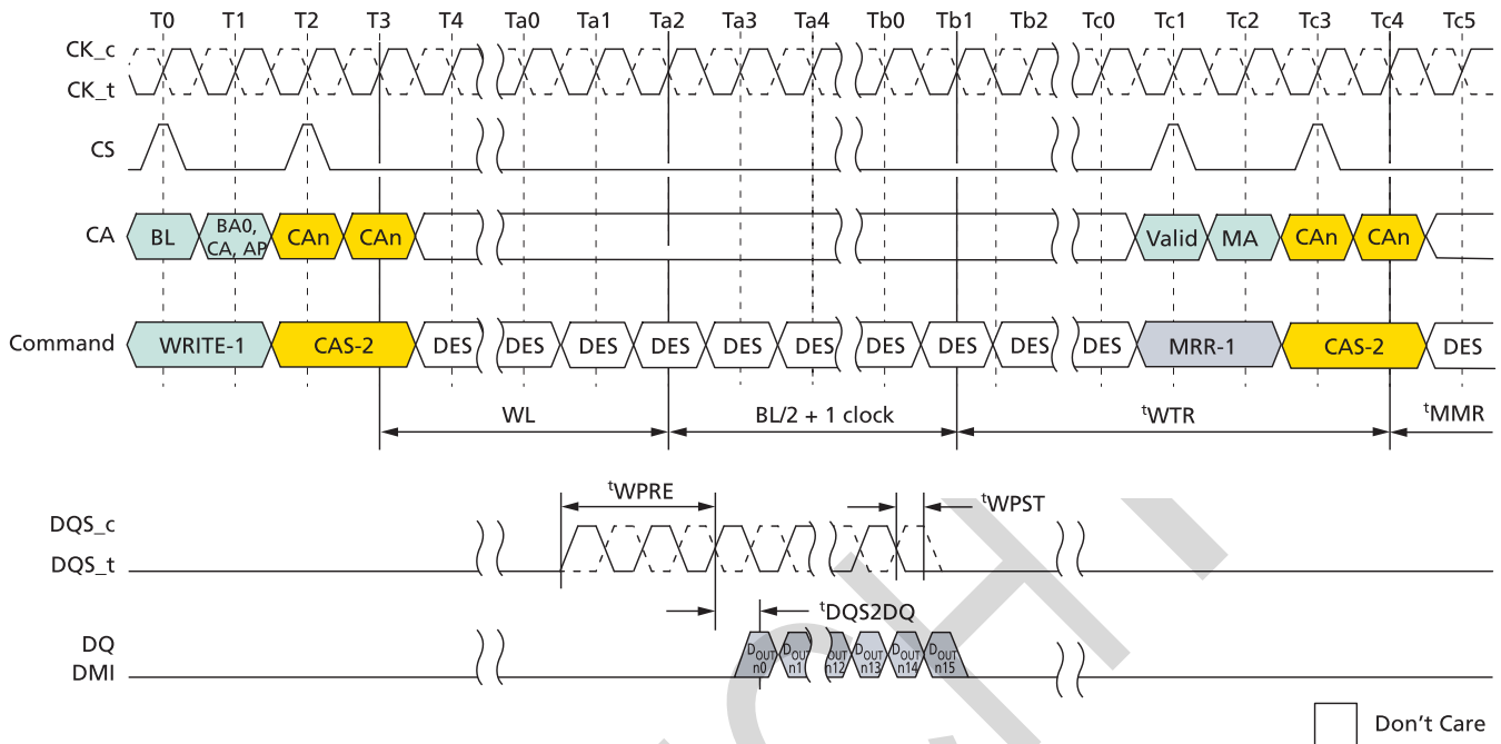
Figure 93: WRITE-to-MRR Timing
