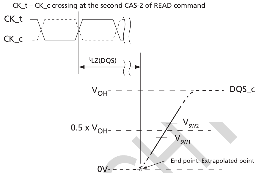
Figure 22: t_{LZ}(DQS) Method for Calculating Transitions and Endpoint
