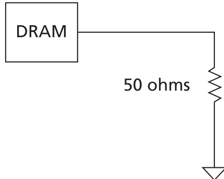
Figure 162: Driver Output Timing Reference Load
