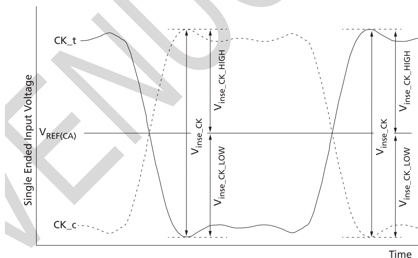
Figure 151: Clock Single-Ended Input Voltage
