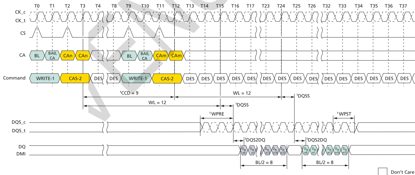
Figure 56: Consecutive WRITE: t_{CCD} = \text{MIN} + 1, 1.5nCK Postamble
