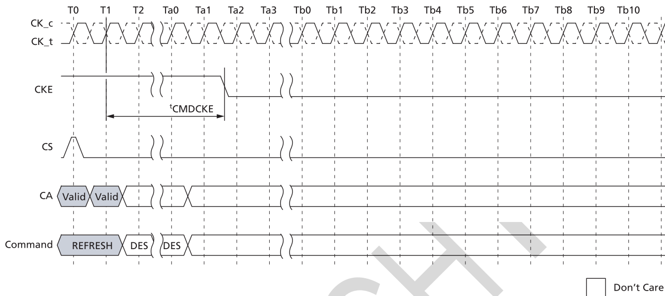
Figure 85: Refresh Entry to Power-Down Entry
