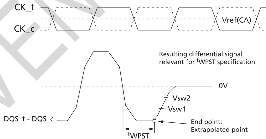
Figure 30: Method for Calculating t_{WPST} Transitions and Endpoints
