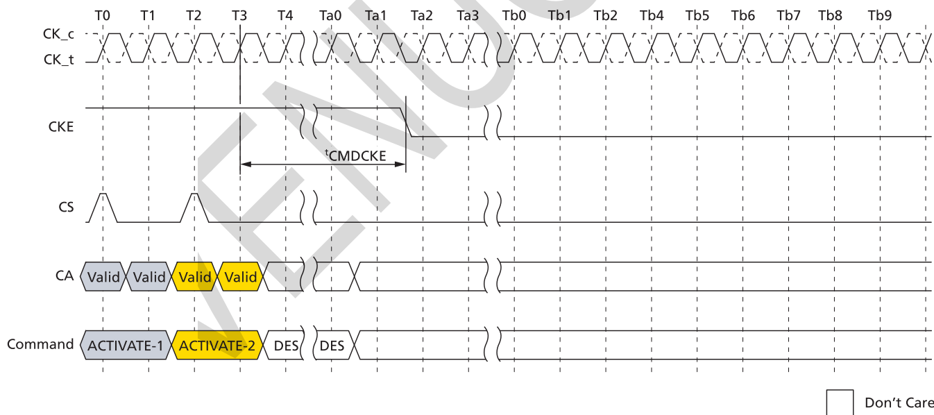
Figure 86: ACTIVATE Command to Power-Down Entry
