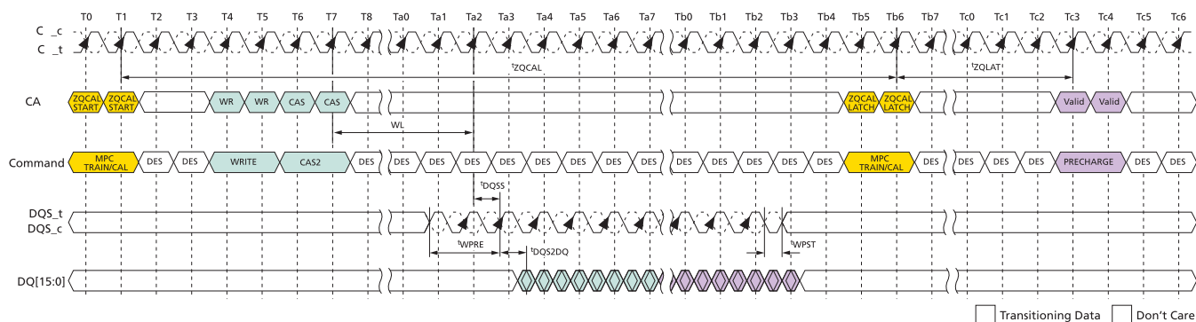
Figure 135: ZQCAL Timing
