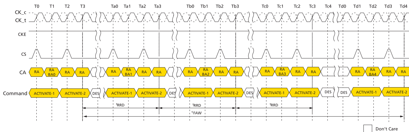
Figure 13: t_{FAW} Timing
