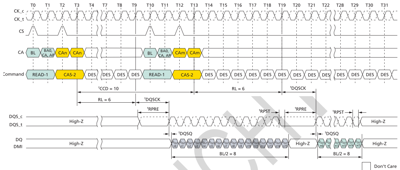
Figure 47: Consecutive READ: t_{CCD} = MIN + 2 , Preamble = Static, 0.5nCK Postamble
