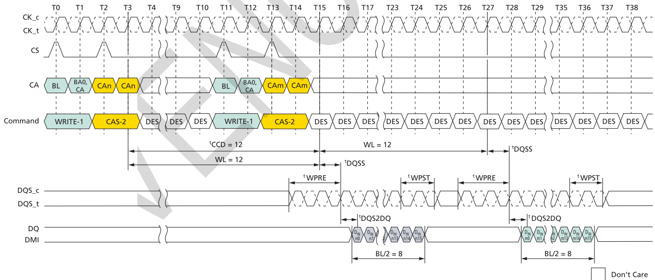
Figure 61: Consecutive WRITE: t_{CCD} = \text{MIN} + 4, 1.5nCK Postamble
