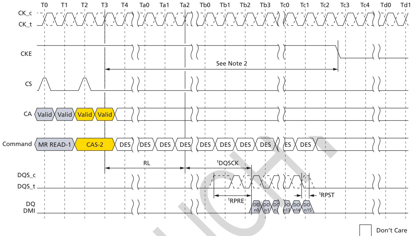
Figure 88: Mode Register Read to Power-Down Entry
