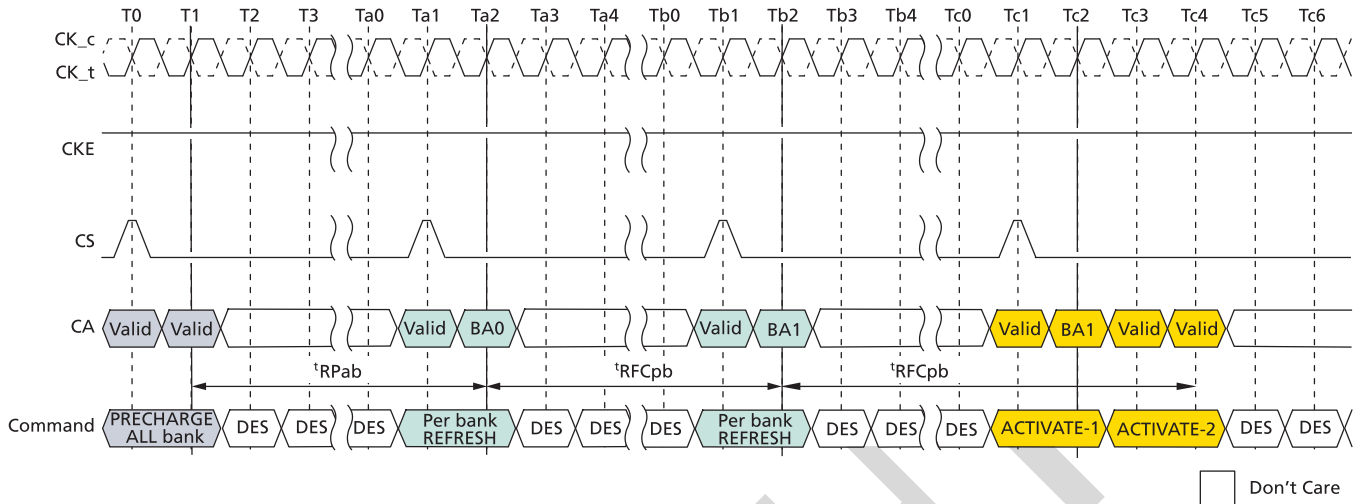
Figure 71: Per Bank REFRESH Operation
