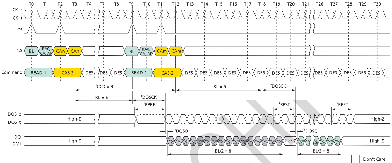
Figur 42: Consecutiv READ: t_{\text{CCD}} = \text{MIN} + 1 , Preamble = Static, 1.5n\text{CK} Postamble
