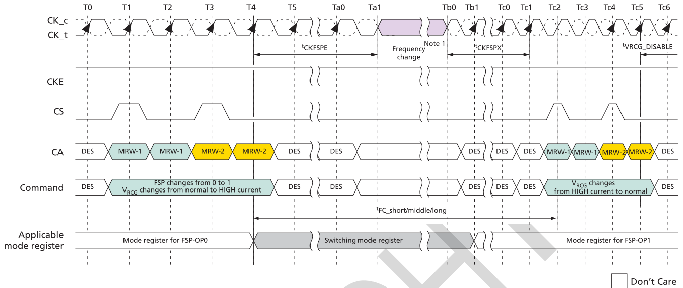
Figure 136: Frequency Set Point Switching Timing
