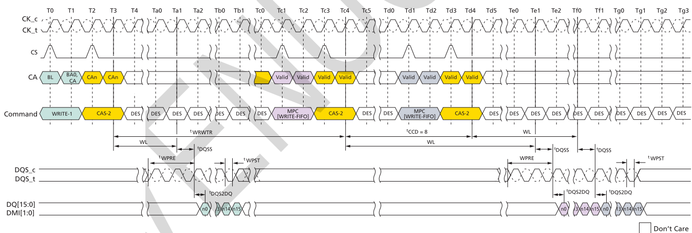
Figure 120: WRITE-FIFO – t_{WPRE} = 2nCK , t_{WPST} = 0.5nCK
