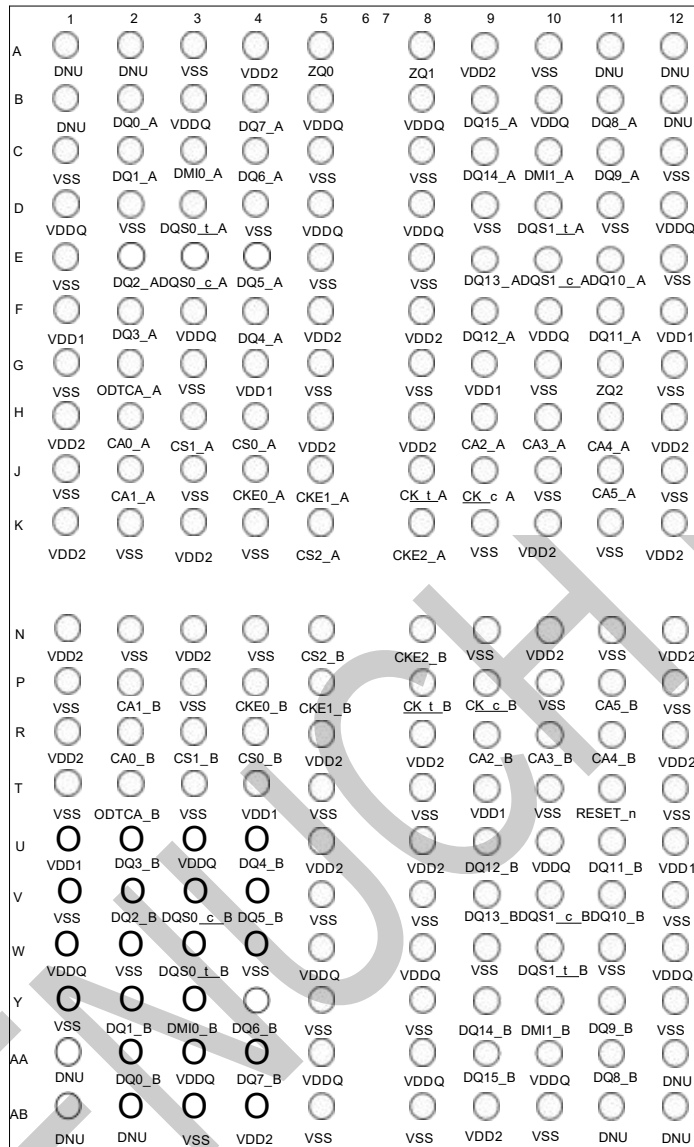
Figure 2-2 x32 Discrete Package Ballout
