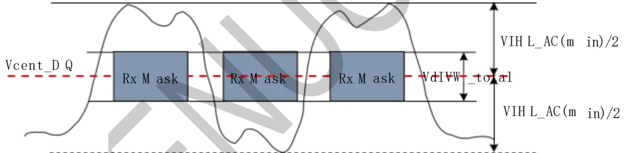
Figure 8-12 DQ VIHL_AC definition (for Each Input Pulse)
