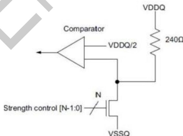
Figure 5-17 Pull-down Calibration
