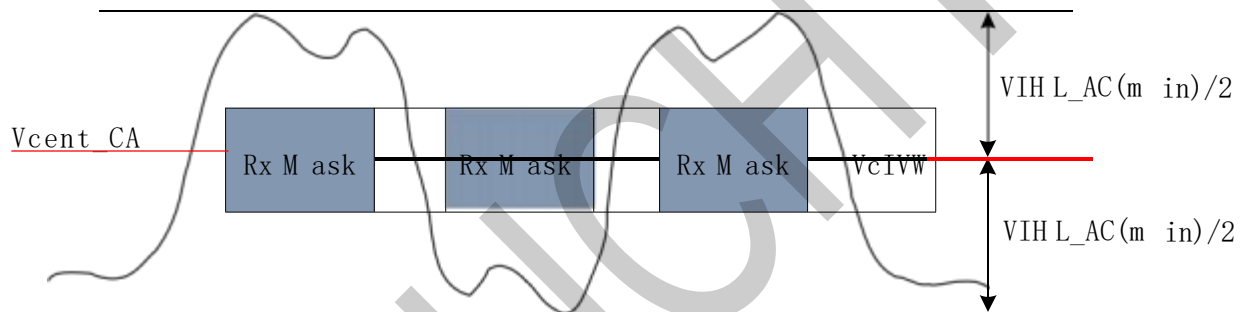
Figure 8-5 CAVIHL_AC Definition (for Each Input Pulse)
