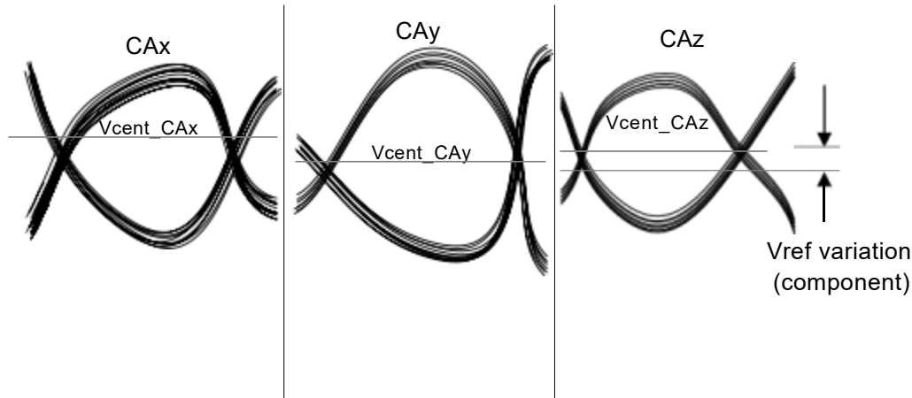
Figure 8-2 Across Pin VREFCA Voltage Variation
